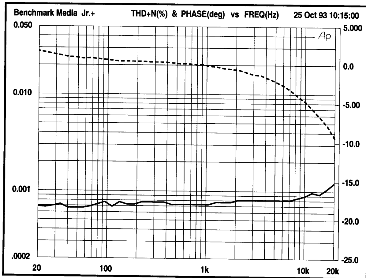
Figure 1. Typical Total Harmonic Distortion and Phase
