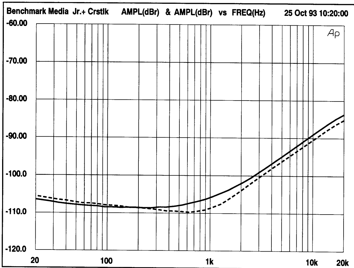
Figure 2. Typical Crosstalk, L into R, and R into L
