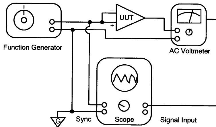
Fig. 2 - Common Mode Rejection Adjustment
