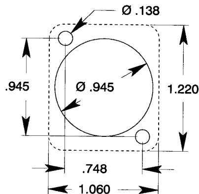
Fig 3.1 Neutrik "D" Series Panel Layout
