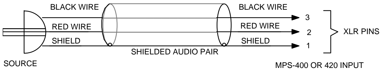
Figure 4 - Unbalanced Output to MPS-400 or MPS-420 Input
