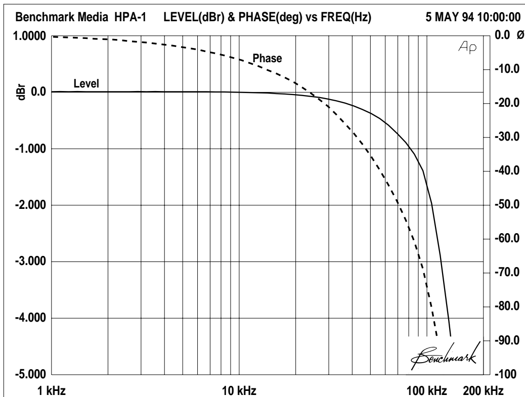
Figure 12 - Amplitude & Phase vs. Frequency. Unity Gain - 0 dB, 200 \Omega load
