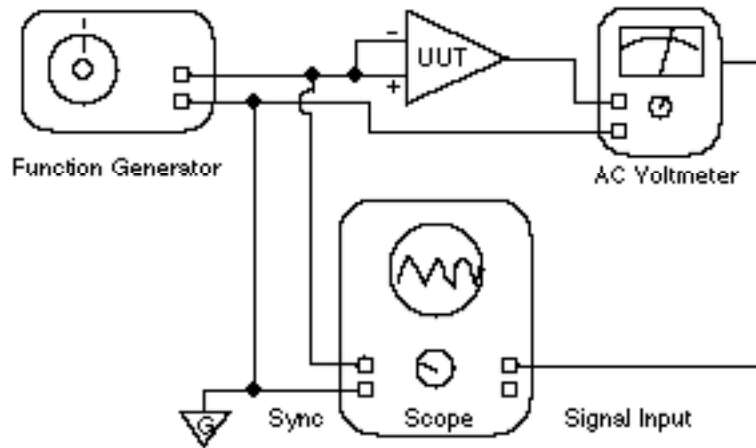
Figure 4 - Common Mode Rejection Adjustment
