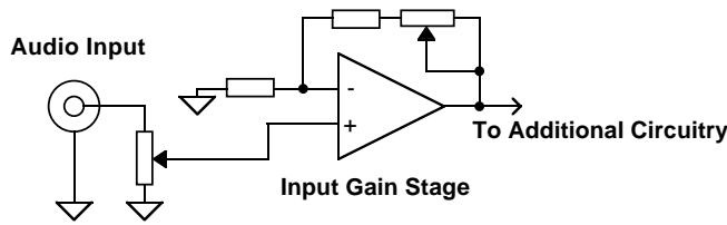
Figure 3 A Common Input Stage
