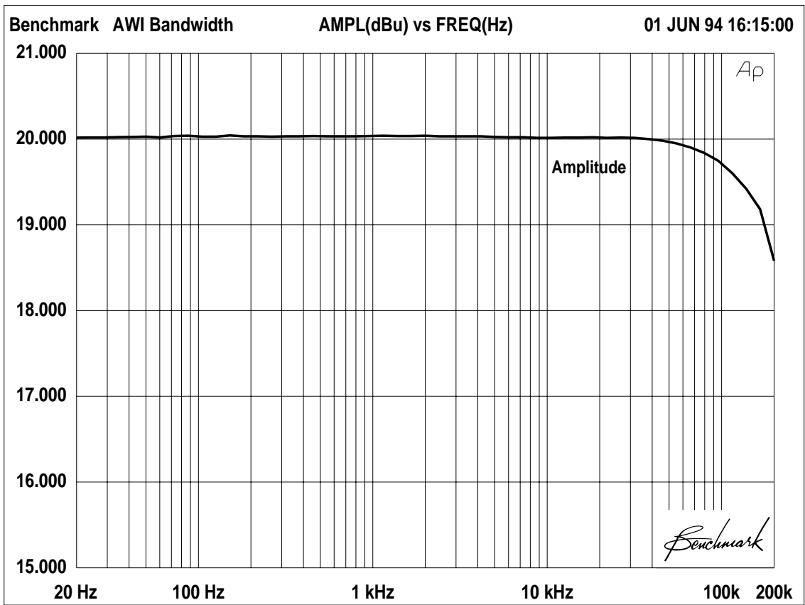
Figure 4. Amplitude Response
