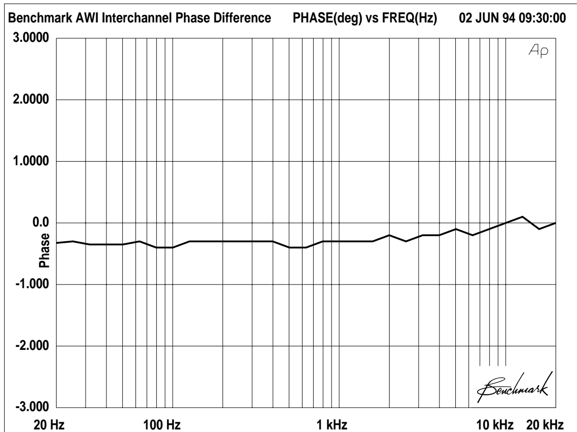
Figure 5. Differential Phase Response
