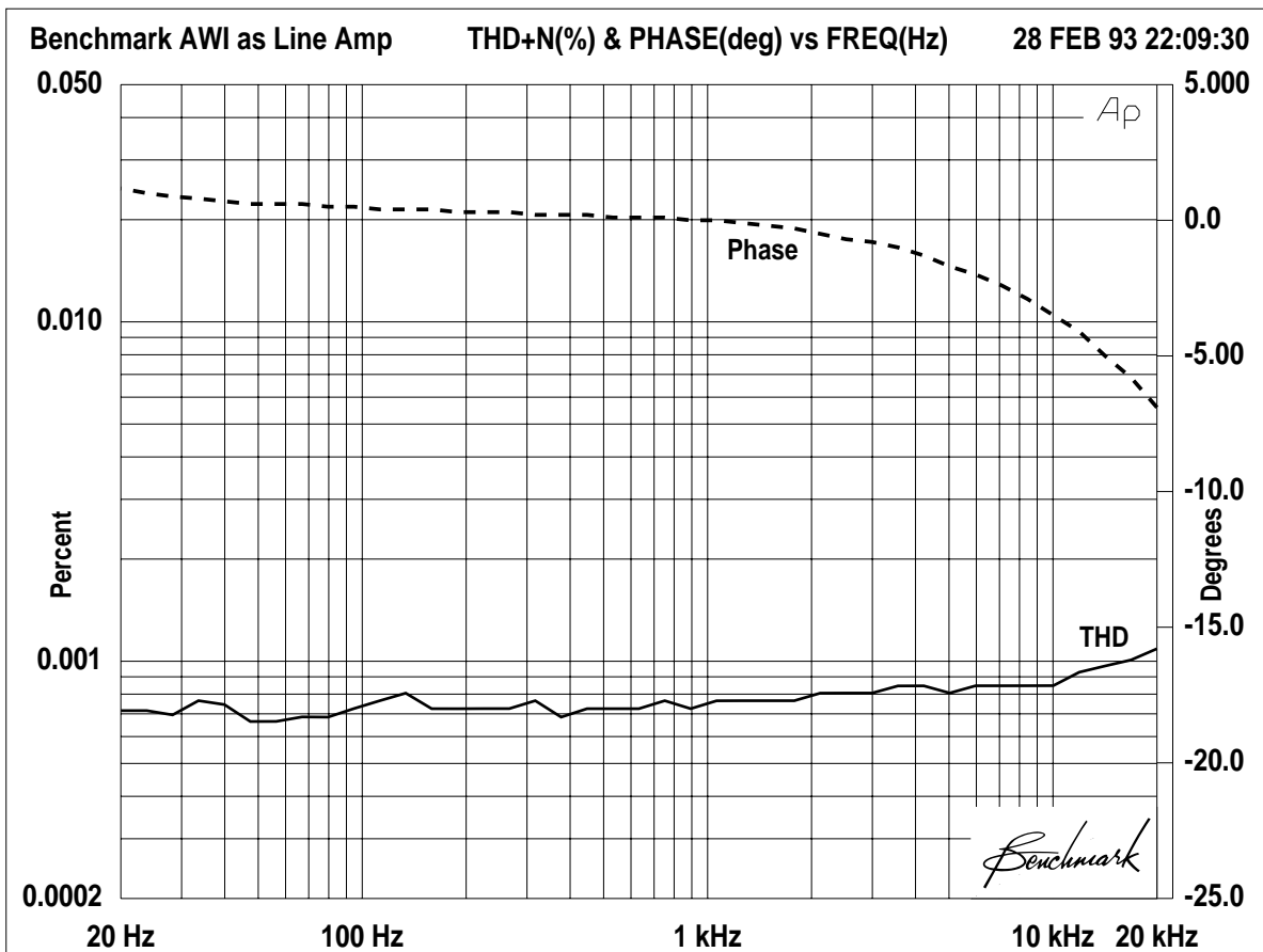
Figure 1. Total Harmonic Distortion and Phase of the AWI as a Line Amp
