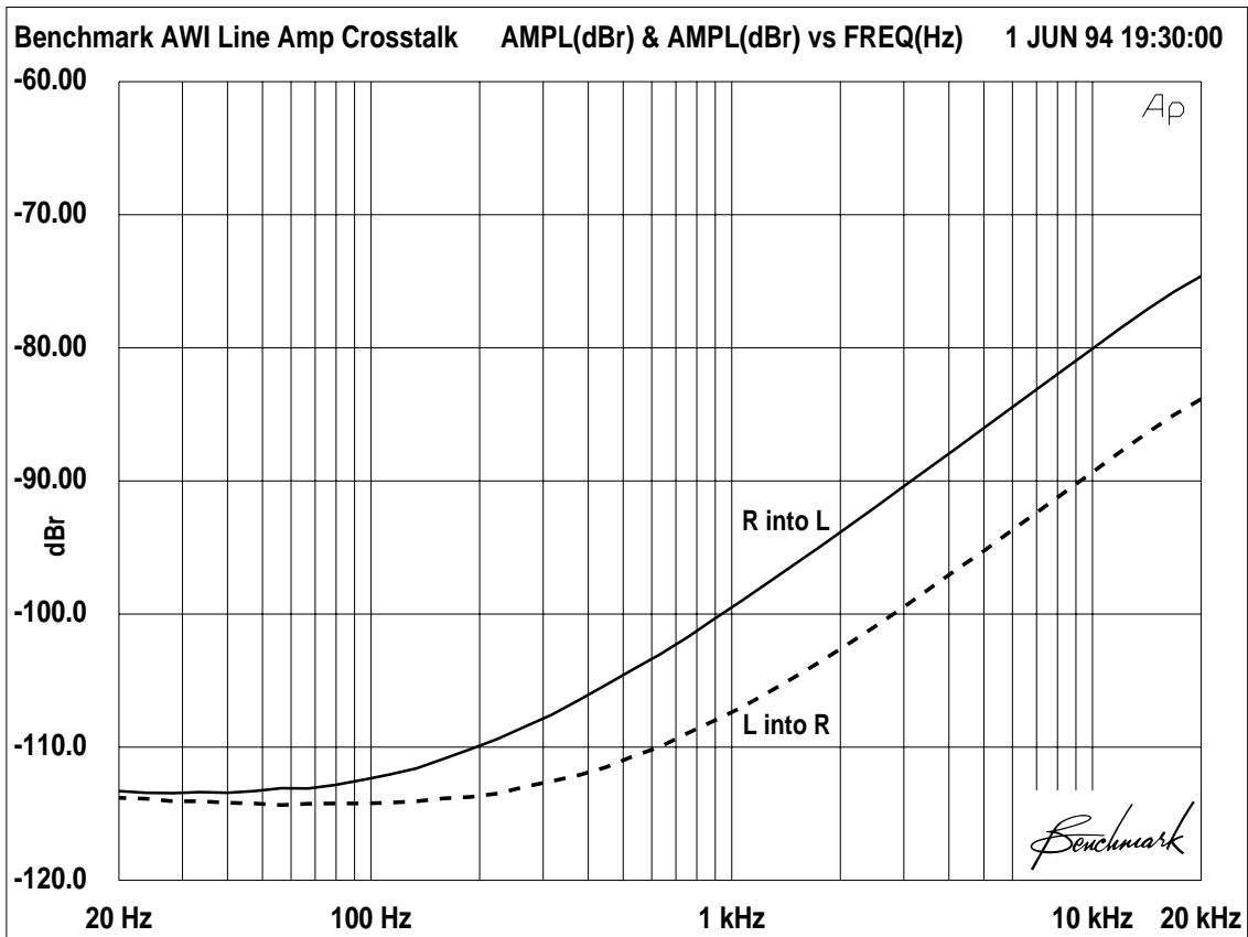
Figure 2. Typical Crosstalk Performance - Line Amp Mode, L into R, and R into L
