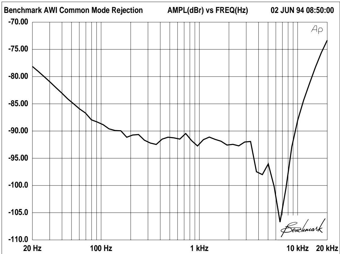
Figure 3. Typical Common Mode Rejection Performance
