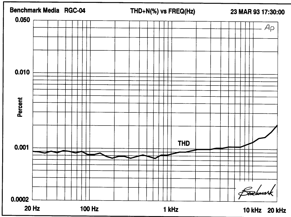
Figure 2. RGC-04 Total Harmonic Distortion at + 20 dBu Out
