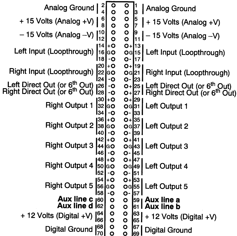
Figure 1. DA-102 Card Edge Connector (Rear View) Showing Aux.0 Line Inputs
